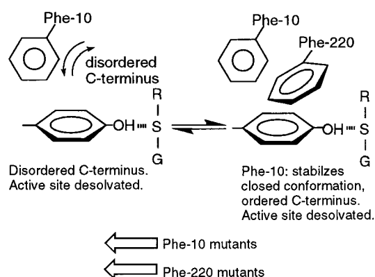
FIGURE 6: Schematic summary of the contribution of Phe-10 to conformational dynamics of the apoenzyme and the complex with a GSH conjugate (R–S–G). Phe-10 directly lowers the pK_a of Tyr-9 in the apoenzyme via edge-to-face interactions. When this interaction is intact, the disordered C-terminus is prevented from sampling conformational space directly over the active site. Phe-10 also stabilizes the closed conformation of the C-terminus in the GSH conjugate complex through interactions with Phe-220. The effects of hydrostatic pressure (from ref 21) and mutations at Phe-10 and Phe-220 (from refs 21 and 22) are summarized. The mutant F220Y is an exception. This mutant stabilizes the closed conformation.
