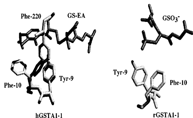
FIGURE 1: Local dynamics of GSTA1-1 near the catalytic Tyr-9. Left: In the apo hGSTA1-1, Phe-10 (black) is above Tyr-9 (black), and the C-terminus is disordered (not visible). Upon addition of the ethacrynic acid conjugate GS-EA, Phe-10 moves to allow Phe-220 within the C-terminal helix to occupy the space above Tyr-9 (structures taken from refs 16 and 17). Right: The Phe-10/Tyr-9 interaction in the rGSTA1-1-GSO 3 - complex (18) is similar to that of the human isoform, except the Phe-10 makes a steeper angle with, and is closer to, the center of the aromatic ring of Tyr-9.
