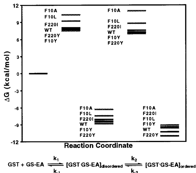
FIGURE 5: Free energy diagram for the reaction coordinate of Phe-10 and Phe-220 mutants. The free energies of the individual proteins have been normalized in the ligand-free state (left).
